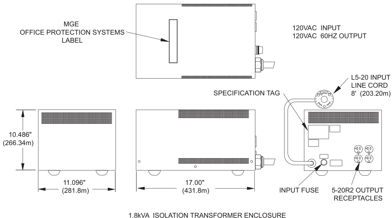
Figure 1-4: 1.8kVA Isolation Transformer Enclosure.
