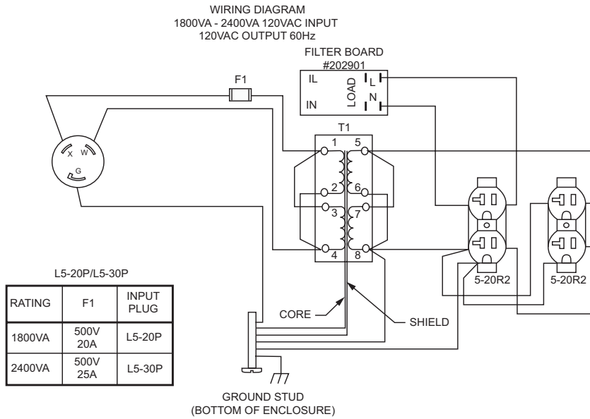
Figure 2-2: Wiring Diagram for 1800VA-2400VA 120VAC Input.
