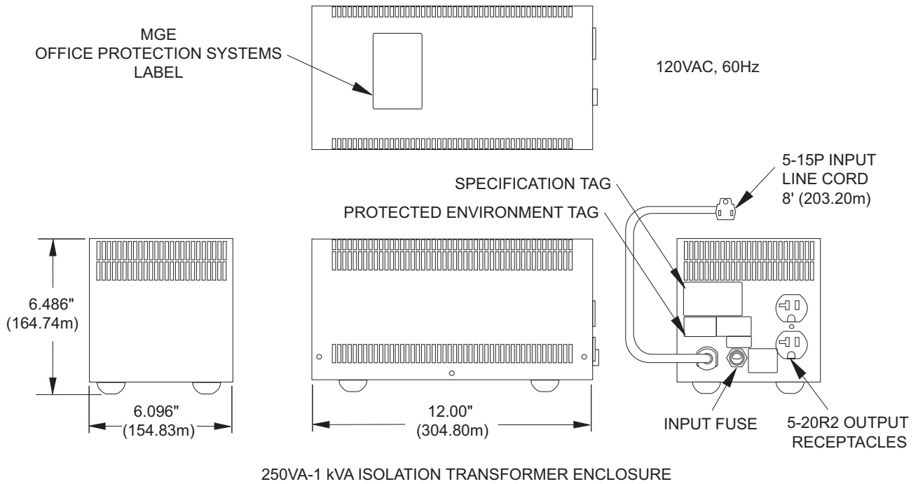
Figure 1-2: 250VA-1kVA Isolation Transformer Enclosure.
