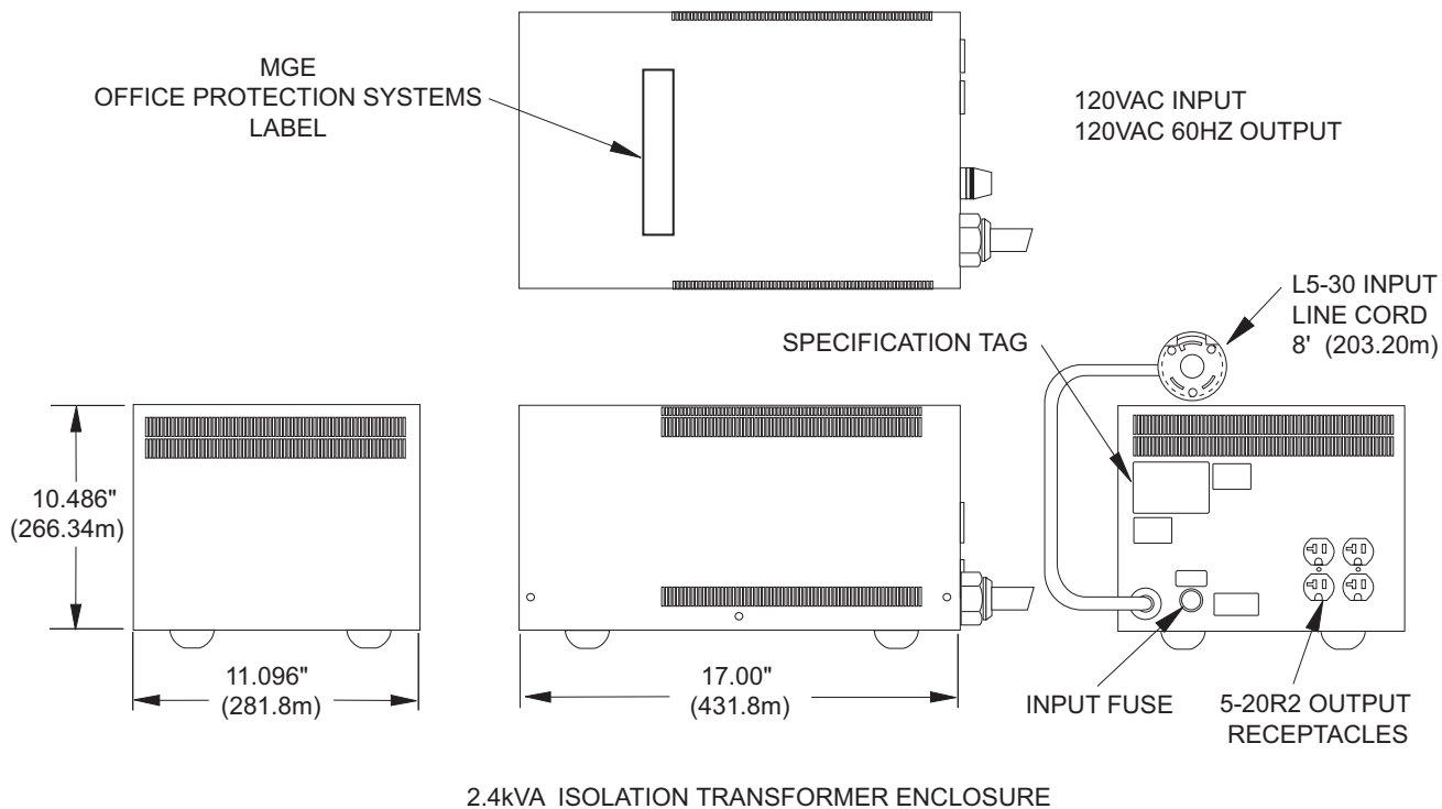
Figure 1-5: 2.4kVA Isolation Transformer Enclosure.
