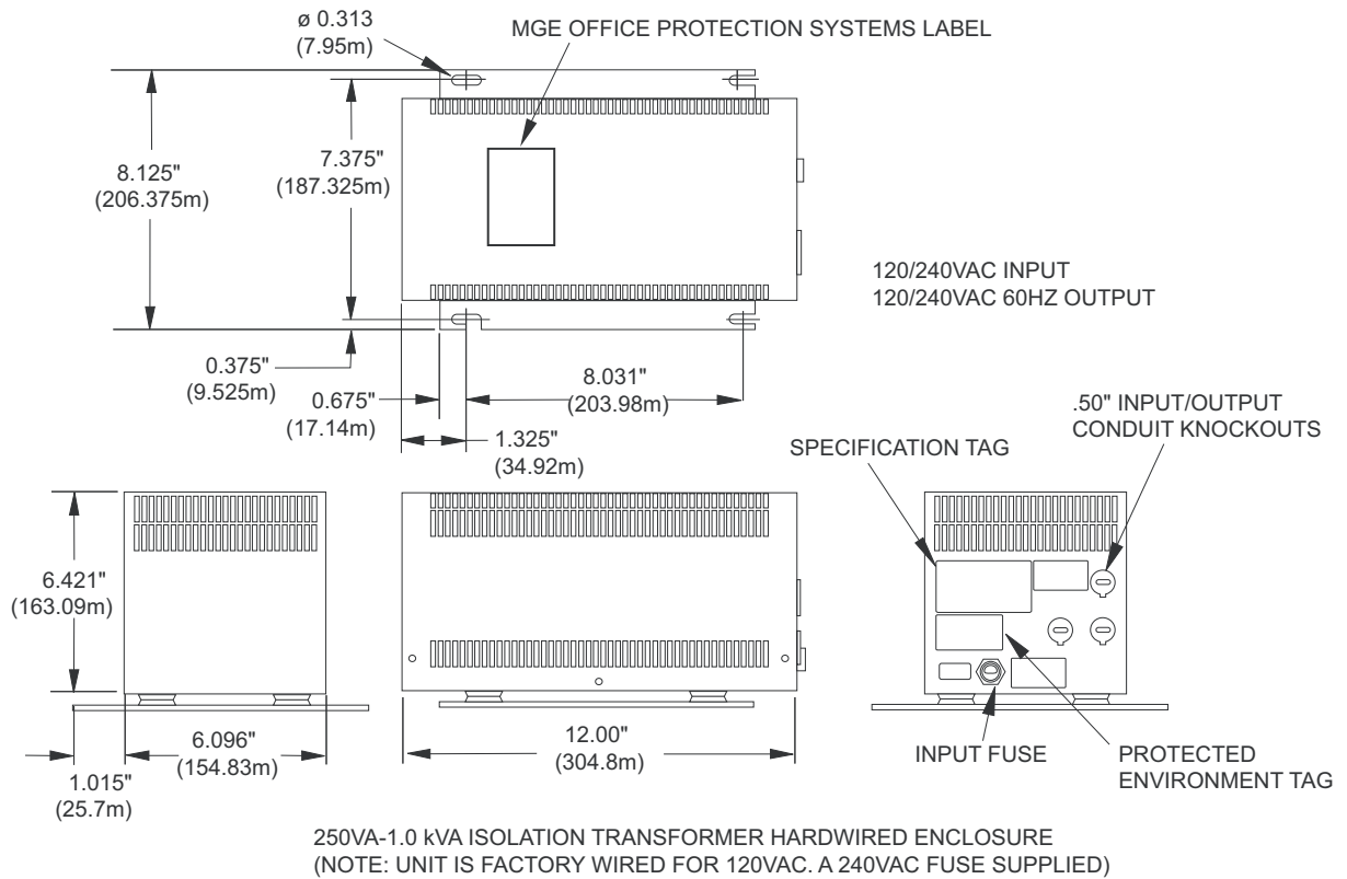
Figure 1-3: 250VA-1kVA Isolation Transformer Hardwired Enclosure.
